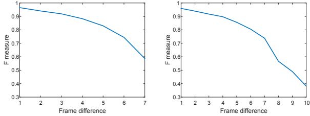
Figure 9. F measure: the success of our algorithm in partitioning the set of candidate matches into inliers and outliers, as a function of the baseline in the sequence for the Herzjesu (left) and Fountain (right) datasets. The inlier ratios are detailed in Table 2.
