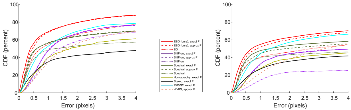
Figure 7. The fraction of pixels mapped by each method to within an error specified on the horizontal axis from their ground truth target location. We present the median for all pairs of images. Dotted lines represent methods disregarding epipolar constraints; dashed lines represent methods using approximate F ; solid lines represent methods using exact F , Herzjesu (left) and Fountain (right).
